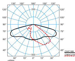
9711SG-AB7L-LR/51/62/75-740 8G2 (7500 lm) TX064277
