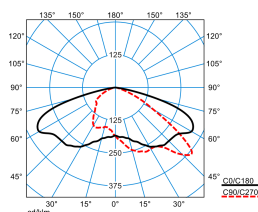
9711SG-AB7L-LR/51/62/75-740 8G2 (6200 lm)
