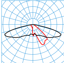
Publisca P1W-AB2L-LRA/2200-730 3G1S TX053497 ■ C0 - C180 ■ C90 - C270 DIN 5040: A30 UTE: 1,00 l DLOR: 100 % ULOR: 0 % CEN Flux Code: 32 69 96 100 100 0 33 67 0
