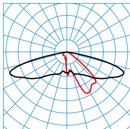
Publisca P1W-AB2L-LRA/2200-730 3G1S ET (CLO initial value) TX300247 ■ C0 - C180 ■ C90 - C270 DIN 5040: A30 UTE: 1,00 l DLOR: 100 % ULOR: 0 % CEN Flux Code: 32 69 96 100 100 0 33 67 0
