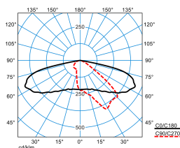
LIQ 50N-AB2L-LR/2600-727 4G1 ET (CLO end value)
