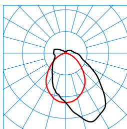
TugraHE 12 PAW 24-75/16ML-840 ET PC 23 (stage 12) TX782007 C0 - C180 C90 - C270
