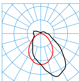
TugraHE 12 PAW 24-75/16ML-840 ET PC 23 (stage 11) TX782004 C0 - C180 C90 - C270
