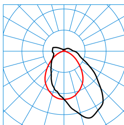
TugraHE 12 PAW 24-75/16ML-840 ET PC 23 (stage 13) TX782010 C0 - C180 C90 - C270
