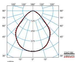
Parelia H-L 13000-840 +LM1 03 (direct c270geo) TX059601
