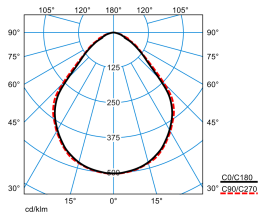
Parelia H-L 13000-840 03 (direct c270geo) TX057120
