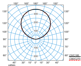
Parelia H-L 13000-840 +LM1 03 (indirect) TX059617
