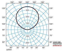
Parelia H-L 13000-840 03 (indirect) TX057122
