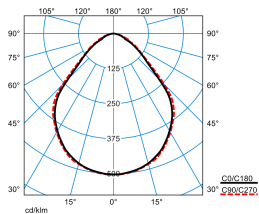
Parelia H-L 13000-840 03 (direct c90geo) TX057121
