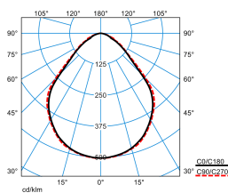
Parella H-L 13000-840 +LM1 03 (direct c90geo) TX059616
