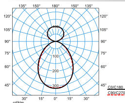
SFlow H3-L MRWD LED6400-8TW ETDD8LLWM 03 (DWW)
