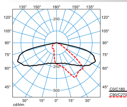
LIQ 50N-AB2L-LRA/5100-740 6G1 ETDD (CLO initial value)
