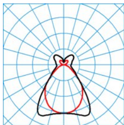
ELINE FL HE PMW1940 840 L150 4 20 ■ C0 - C180 DIN 5040 3 = B52 UGR 1 3 = 13,9 UGR q 3 = 17,0 UTE 3 = 0,72 D + 0,28 T CEN Flux Code 3 = 60 83 94 72 100 26 58 82 28
