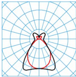
ELINE FL HE PMW1940 827 L150 2 20 ■ C0 - C180 DIN 5040 = B52 UGR 1 = 13,7 UGR q = 16,8 UTE = 0,72 D + 0,28 T CEN Flux Code = 60 83 94 72 100 26 58 82 28
