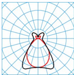
ELINE FL HE PMW1940 865 L150 3 20 ■ C0 - C180 DIN 5040 2 = B52 UGR 1 2 = 13,9 UGR q 2 = 17,0 UTE 2 = 0,72 D + 0,28 T CEN Flux Code 2 = 60 83 94 72 100 26 58 82 28
