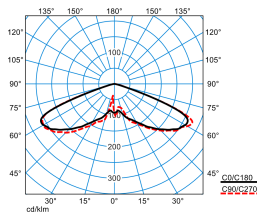
Publisca P1-RB6L/2400-730 3G1S ETDD (CLO end value) TX301588 DIN 5040: A20 UTE: 1,00 J DLOR: 100 % ULOR: 0 % CEN Flux Code: 20 57 98 100 100
