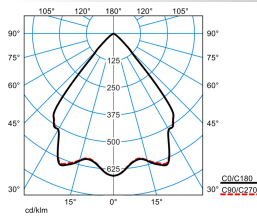
ELINE HE CLW22100 830 L150 1 20
