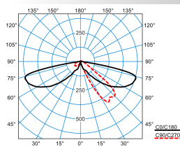
8841 AB2L/700-730 2G2 ETDD (CLO initial value)
