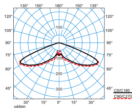
Publisca P1W-RB6L/3200-730 4G1S ETDD (CLO end value)
