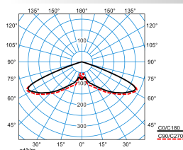
Publisca P1W-RB6L/3200-730 4G1S ETDD (CLO initial value)
