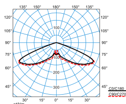
Publisca P1W-RB6L/3200-730 4G1S
