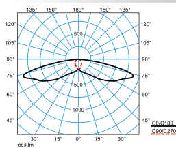
LIQ 50N-SB3L-LRA/1800-740 2G1 ETDD (CLO initial value)
