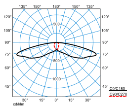
LIQ 50N-SB3L-LRA/1800-740 2G1 ETDD (CLO end value)
