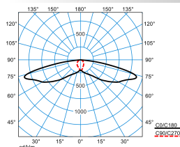
LIQ 50N-SB3L-LR/1650-722 2G1 ET (CLO initial value)
