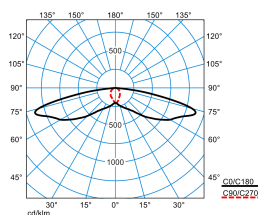
LIQ 50N-SB3L-LRA/1500-730 2G1 ETDD (CLO end value)
