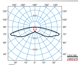
LIQ 50N-SB3L-LRA/1500-730 2G1 ETDD (CLO initial value)
