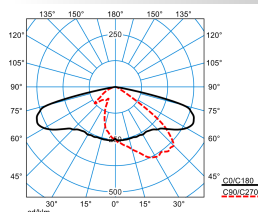
LIQ 70N-AB7L-LRA/12000-730 12G1 ETDD(CLO initial value)
