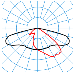
LIQ 70N-AB7L-LRA/12000-730 12G1 ETDD(CLO initial value) TX277690
