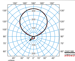
Luceos S-U PAW-IL 300-830 ETDI 03+LLWP (LEO2)
