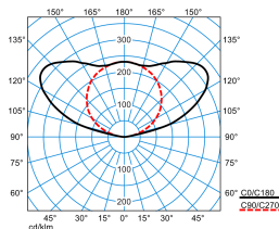
E-Line PRO 78HE I-UW 30-830ETDD L75 05 05
