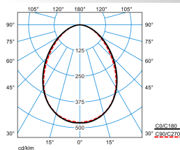
SFlow D2-L MRWD LED4000-830 ET 01
