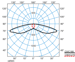
LIQ 50N-SB3L-LR/1350-730 2G1 ET (CLO initial value)
