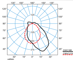
TugraHE 21 PAW 79-130/16ML-840 ET PC 23 (stage 0) TX781307
