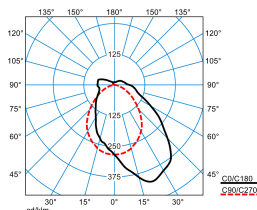
TugraHE 21 PAW 79-130/16ML-840 ET PC 23 (stage 1) TX781310
