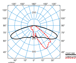
Publisca P2-AB2L/4200-730 6G1S ETDD (CLO initial value)
