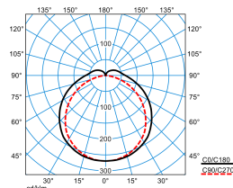
Deveo G3 6 DL 10-30/3ML-8MC ET PC (stage 6)
