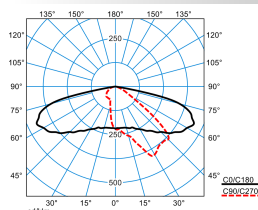
LIQ 50N-AB2L-SLR2/6800-730 6G1 ET (CLO initial value)
