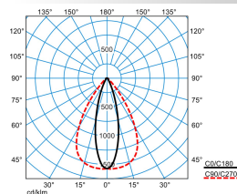
78IP50 HE+ LEN80 830 L150 1 50
