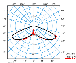
Publisca P1-RB6L/2600-730 3G1S ETDD (CLO initial value) TX300978 DIN 5040: A20 UTE: 1,00 J DLOR: 100 % ULOR: 0 % CEN Flux Code: 20 57 98 100 100
