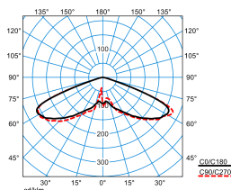
Publisca P1-RB6L/2600-730 3G1S ETDD (CLO end value) TX300259 DIN 5040: A20 UTE: 1,00 J DLOR: 100 % ULOR: 0 % CEN Flux Code: 20 57 98 100 100
