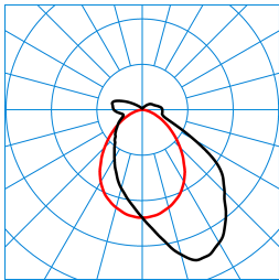
TugraHE Act 18 PAW 70-840 ETDD8 01 (ACTDCW) TX303169 ■ C0 - C180 ■ C90 - C270 DIN 5040: B40 UTE: 0.87 E + 0.13 T DLOR: 87 % ULOR: 13 % CEN Flux Code: 48 79 93 87 100 7 25 60 13
