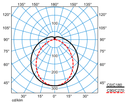
So-Tube G3 D/H4 DW 40-840 ETDD 05 TX773678
