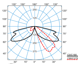
LTX L-AB2C-SLR1/1800-730 4G1ET (CLO end value)
