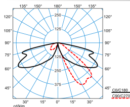
LTX L-AB2C-SLR1/1800-730 4G1ET (CLO initial value)
