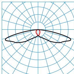
LIQ 50N-SB3L-SLR1/2200-722 2G1 ET (CLO initial value) TX779344 ■ C0 - C180 ■ C90 - C270 DIN 5040: A30 UTE: 1,00 l DLOR: 100 % ULOR: 0 % CEN Flux Code: 31 64 92 100 100
