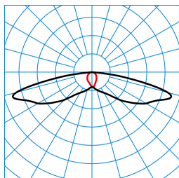
LIQ 50N-SB3L-SLR1/2200-722 2G1 ET (CLO end value) TX779339 ■ C0 - C180 ■ C90 - C270 DIN 5040: A30 UTE: 1,00 l DLOR: 100 % ULOR: 0 % CEN Flux Code: 31 64 92 100 100
