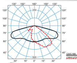
LIQ 70N-AB7L-LR/12000-722 12G1 ET (CLO initial value)
