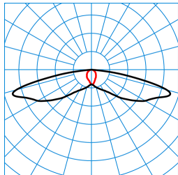
LIQ 50N-SB3L-LR/1800-730 2G1 ET (CLO end value) TX776044 ■ C0 - C180 ■ C90 - C270 DIN 5040: A30 UTE: 1,00 l DLOR: 100 % ULOR: 0 % CEN Flux Code: 31 64 92 100 100
