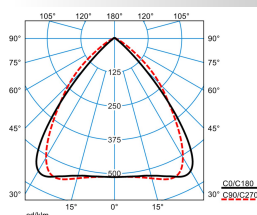
ELINE LN40-110 ML 865 L150 0 20
