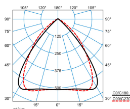
ELINE LN40-110 ML 865 L150 2 20
