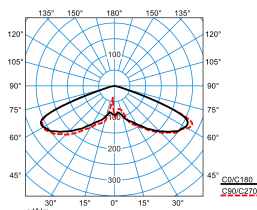
Publisca P1-RB6L-LRA/2400-740 3G1S ET (CLO initial value) TX300910 DIN 5040: A20 UTE: 1,00 J DLOR: 100 % ULOR: 0 % CEN Flux Code: 20 57 98 100 100
