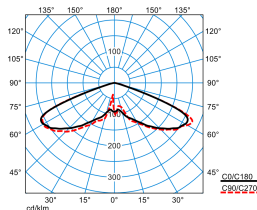
Publisca P1-RB6L-LRA/2400-740 3G1S TX047670 DIN 5040: A20 UTE: 1,00 J DLOR: 100 % ULOR: 0 % CEN Flux Code: 20 57 98 100 100
