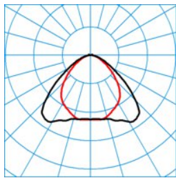
ELINE FL HE LVW120 830 L225 1 20 ■ C0 - C180
