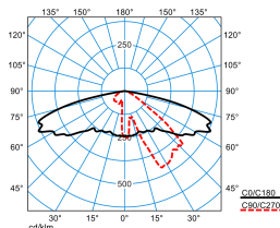
Publisca P1W-AB2L-LRA/1200-730 2G1S
