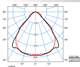
SFlow C3-L MRW LED4000-8TW ETDD8 LLWS 01 (DWW)
