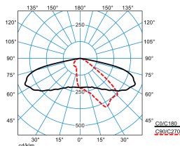
LIQ 50N-AB2L-LR/5600-730 6G1 ET (CLO initial value) TX778002
