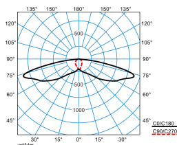
LIQ 50N-SB3L-LRA/1800-730 2G1 ETDD (CLO initial value) TX780314
