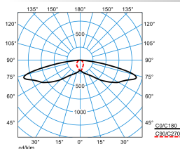
LIQ 50N-SB3L-LRA/1800-730 2G1 ETDD (CLO initial value)
