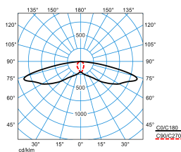
LIQ 50N-SB3L-LRA/1800-730 2G1 ETDD (CLO end value)
