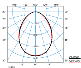
SFlow C1-L MRWD LED3200-830 ET 01
