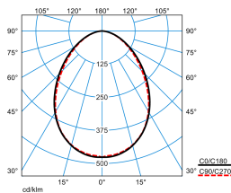
SFlow C1-L MRWD LED3200-830 ET 01 TX721330
