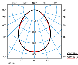
SFlow C1-L MRWD LED3200-830 ET 01 TX771459
