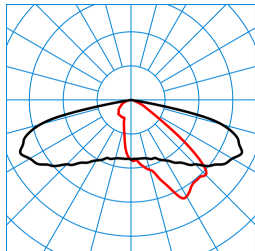
LIQ 50N-AB2L-SLR1/6800-730 6G1 ET (CLO end value) TX777037
