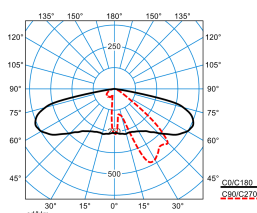
Publisca P2-AB2L-LRA/1000-740 2G1S ET (CLO initial value) TX300328 DIN 5040: A30 UTE: 1,00 G DLOR: 100 % ULOR: 0 % CEN Flux Code: 34 70 96 100 100
