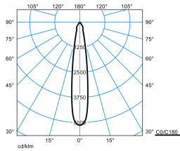
E-Line PRO 78 BV G2 RF-SP 30-BC M49 ETBLE 01 Blank
