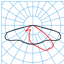
LIQ 70N-AB7L-LRA/9100-727 10G1 ETDD (CLO end value) TX278302
