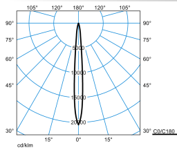
Faciella 20 RE2L/4200-840 1G1 TX044312
