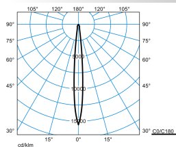
Inveria C 210 RE7R/3100-830 ETBLE +CAS
