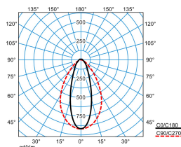
ELINE PN55-120 ML 840 L225 2 20
