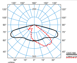
LIQ 70N-AB7L-SLR2/7500-740 8G1 ET(CLO initial value)
