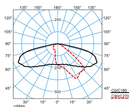
LIQ 50N-AB2L-LRA/3500-727 4G1 ETDD (CLO end value)
