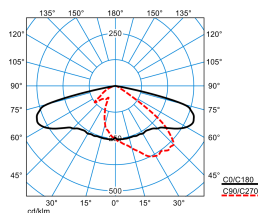
LIQ 70N-AB7L-LRA/10/12/135-727 12G1 ETDD(CLO initial value) TX277990
